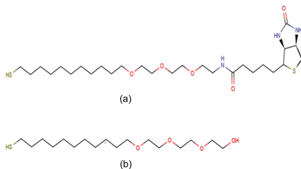
Fig. 1 Molecular structure of (a) biotinylated PEG thiol (SH-[CH 2 ] 11 -EG 3 -Biotin) and (b) OH-terminated PEG thiol (SH-[CH 2 ] 11 -EG 3 -OH).
